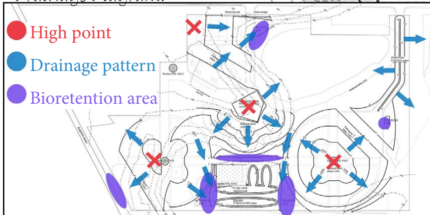
Drainage Diagram:
